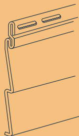
Double 4" Traditional Clapboard Exposure: 8" Length: 12' 6"
