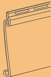
Single 8" Traditional Clapboard Exposure: 8" Length: 12' 6"
